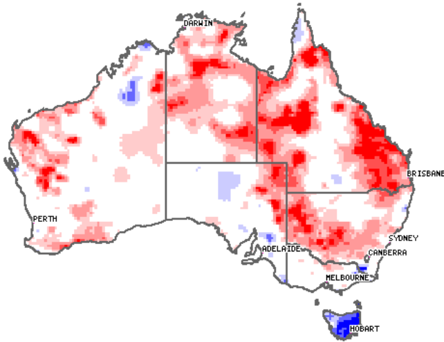
Rainfall percentiles for the last three months August 2009 – October 2009
