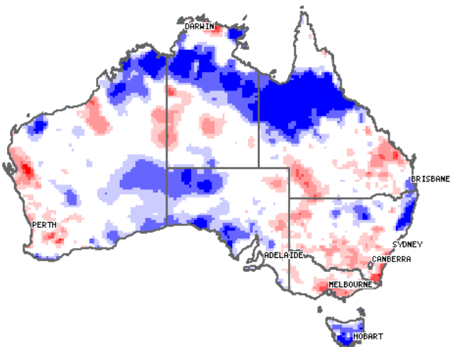
Rainfall percentiles for the last 12 months November 2008 – October 2009
